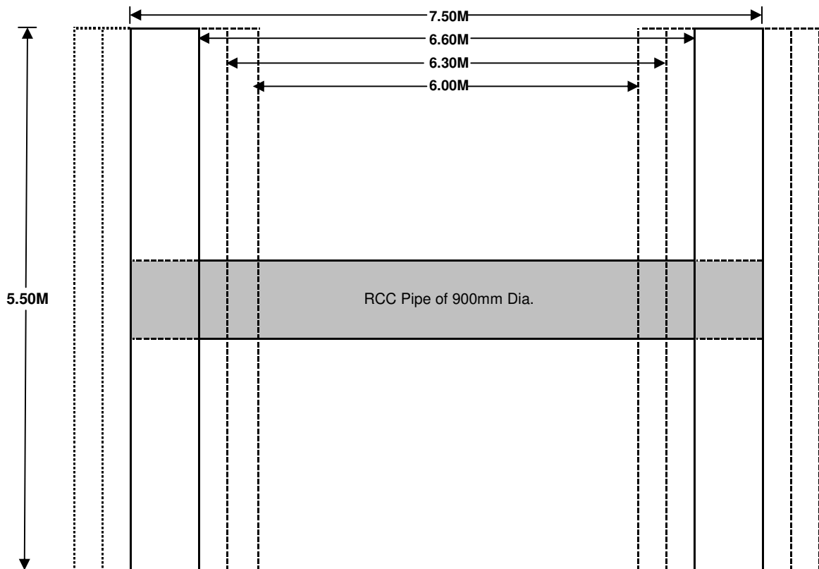
Plan of Culvert
