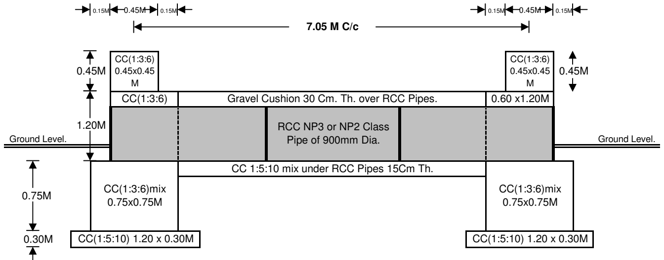
Sectional Elevation
