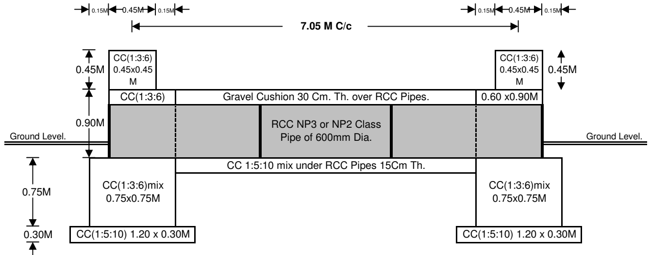
Sectional Elevation
