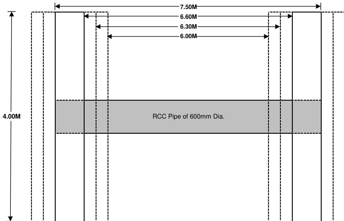
Plan of Culvert
